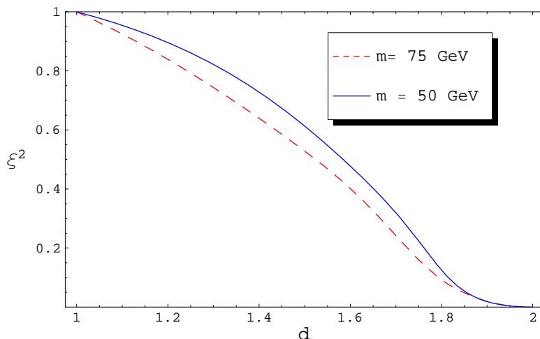
Figure 7. \xi^2 as a function of d for \mu = 100 GeV, m = 75 GeV and \mu = 100 GeV, m = 50 GeV.
