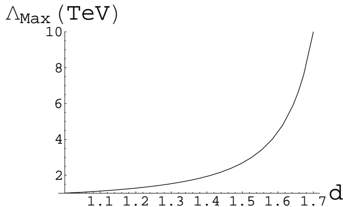
Figure 9. Qualitative behavior of \Lambda_{\text{max}} as a function of d for fixed \mu and \lambda_t .
